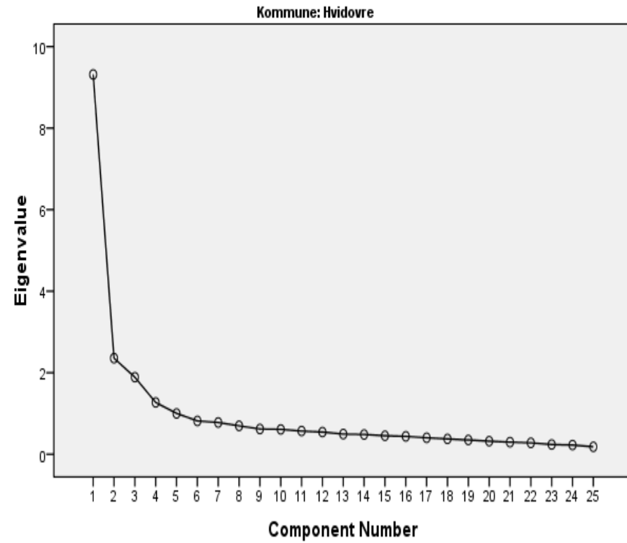
Scree Plot
