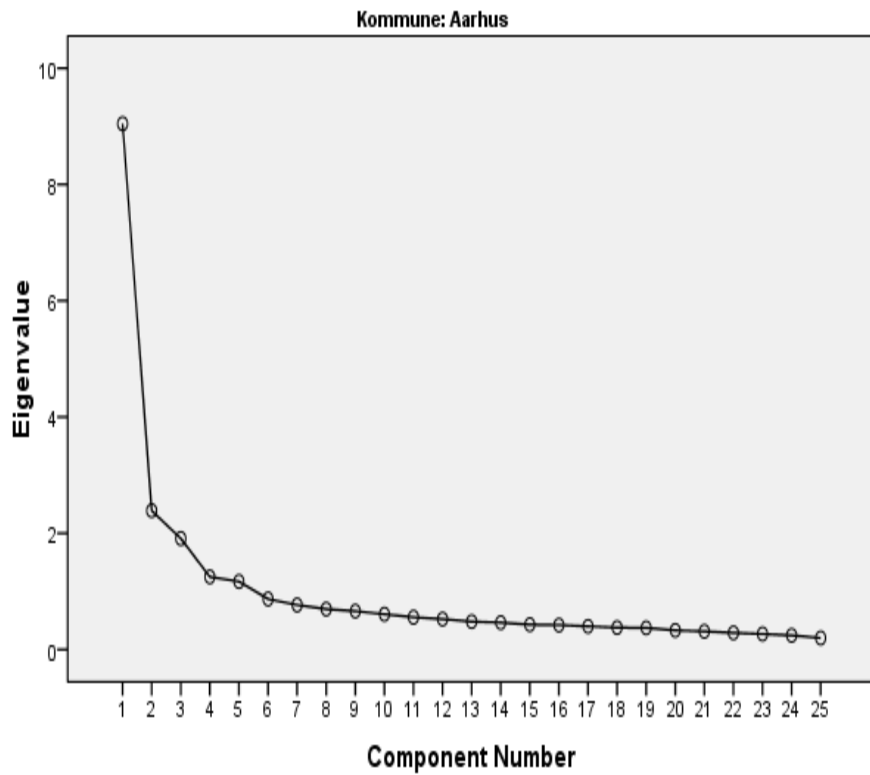
Scree Plot
