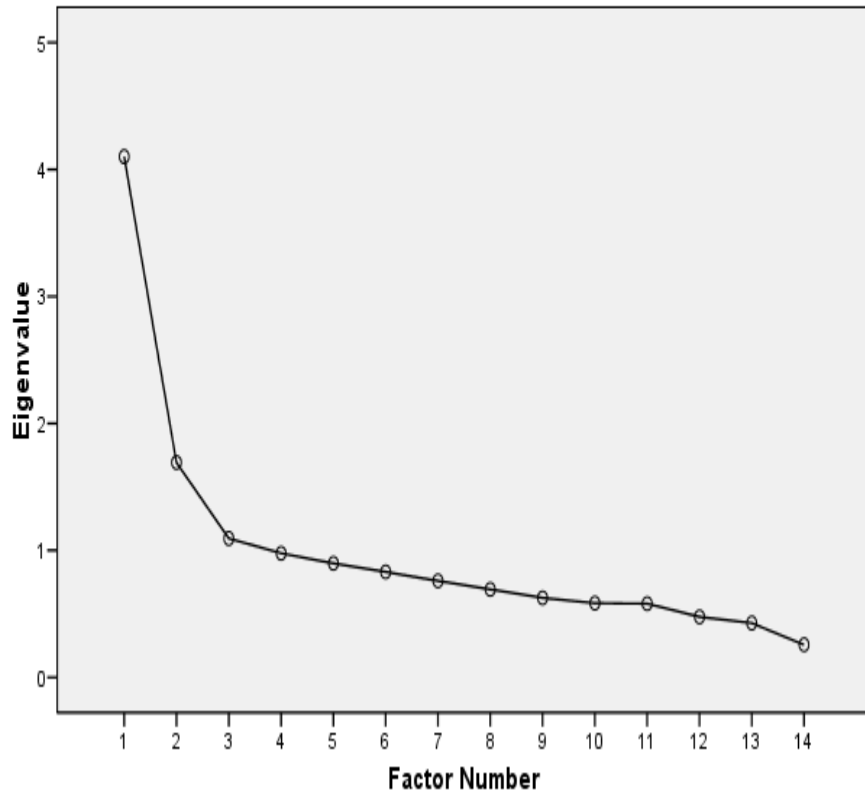
Scree Plot
