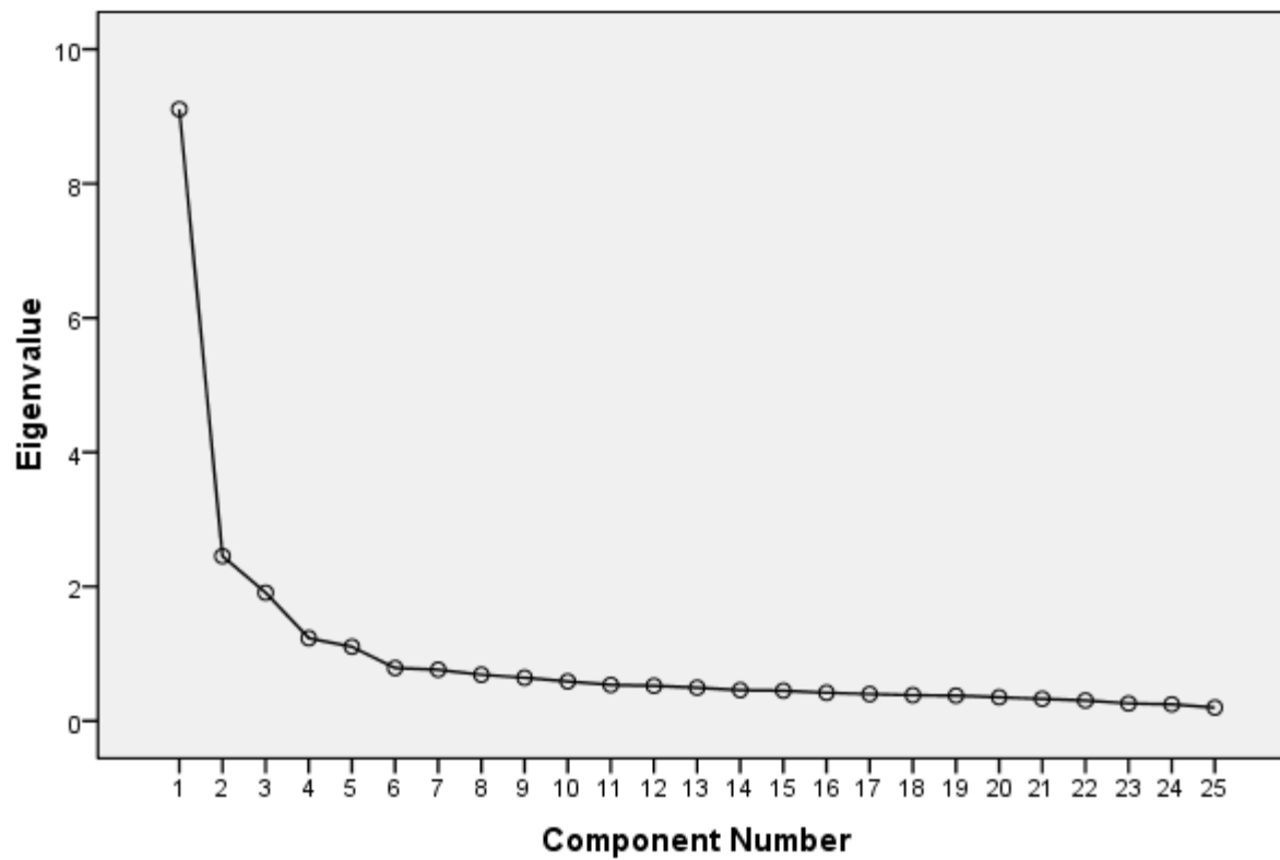
Scree Plot
