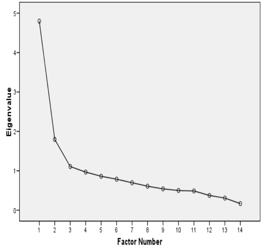
Scree Plot
